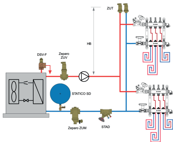
Varmepumpe system
